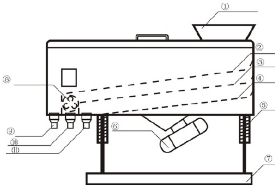
Abridged general view of the machine structure
